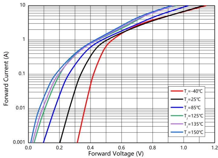
Fig.3: Forward characteristics
