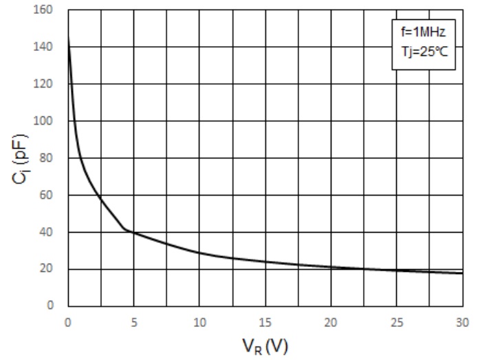
Fig.2: Junction Capacitance
